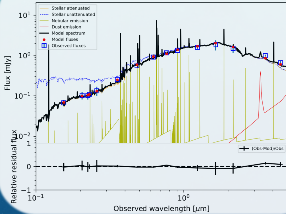
Best model for pix261_258 at z = 0.0 . Reduced \chi^2 = 0.3
